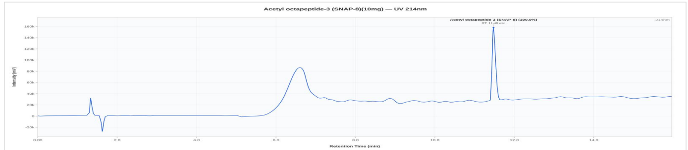
Snap-8 10mg - B10017: UV Chromatogram
